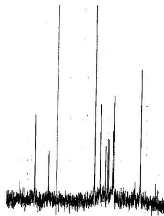
Fig. 2. ^{13}\text{C} NMR of polysaccharides isolated from P. erengii
